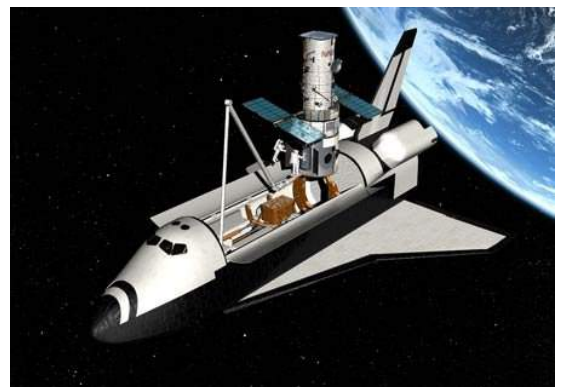
Hubble Space Telescope
