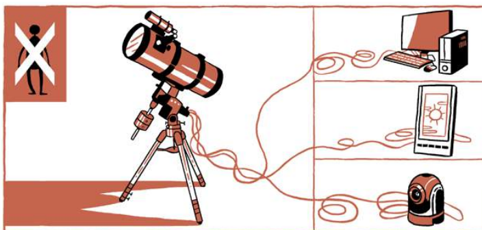
Robotic telescopes
